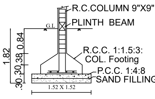
FOUNDATION DETAIL
