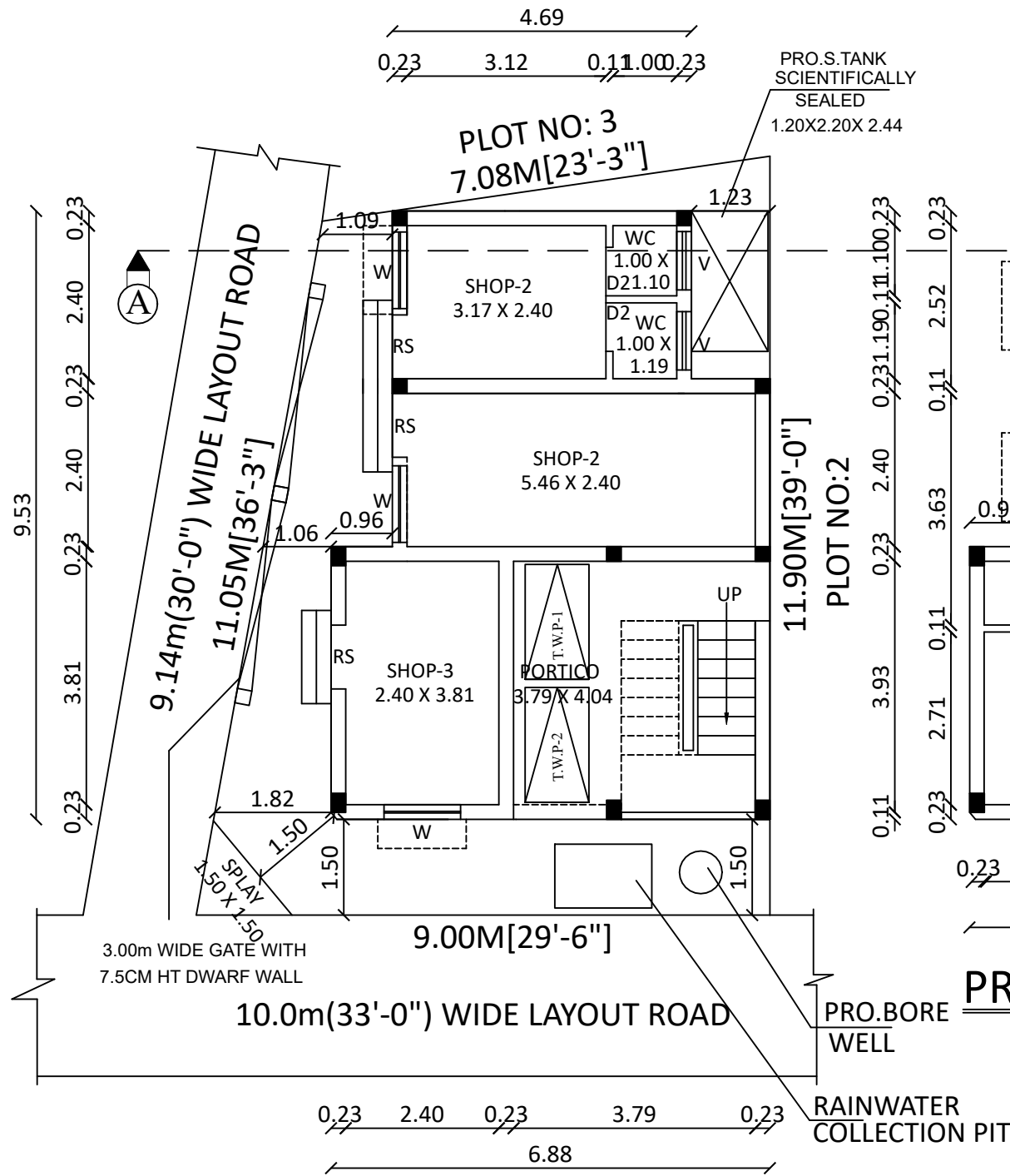
SITE CUM PRO.GROUND FLOOR PLAN
