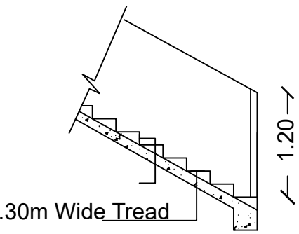
STAIRCASE DETAILS
