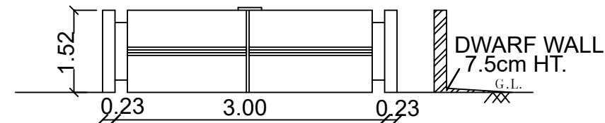
GATE PLAN & ELEVATION
