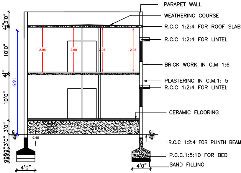
SECTION ON 'SC'
