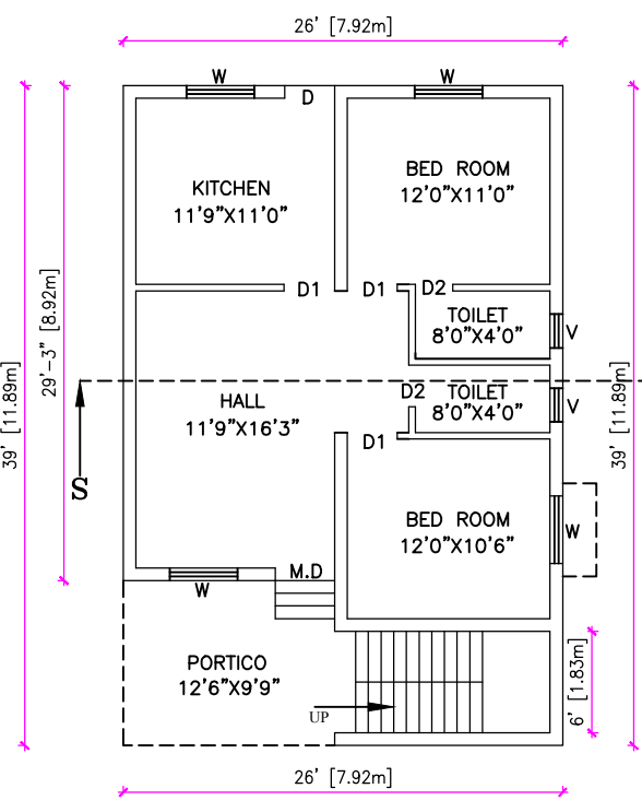
EXTG. GROUND FLOOR PLAN
