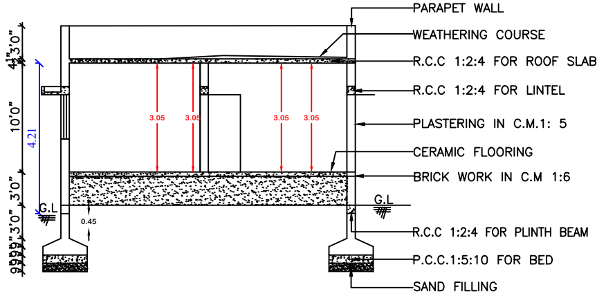
SECTION ON 'SC'
