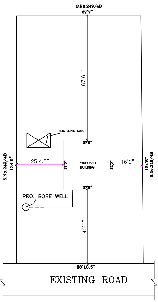
SITE PLAN
