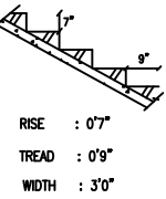
STAIRS DETAILS
