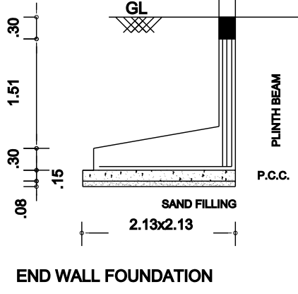
END WALL FOUNDATION
