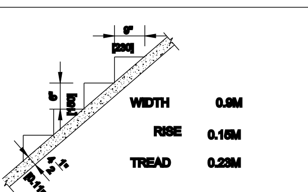
STAIRCASE
