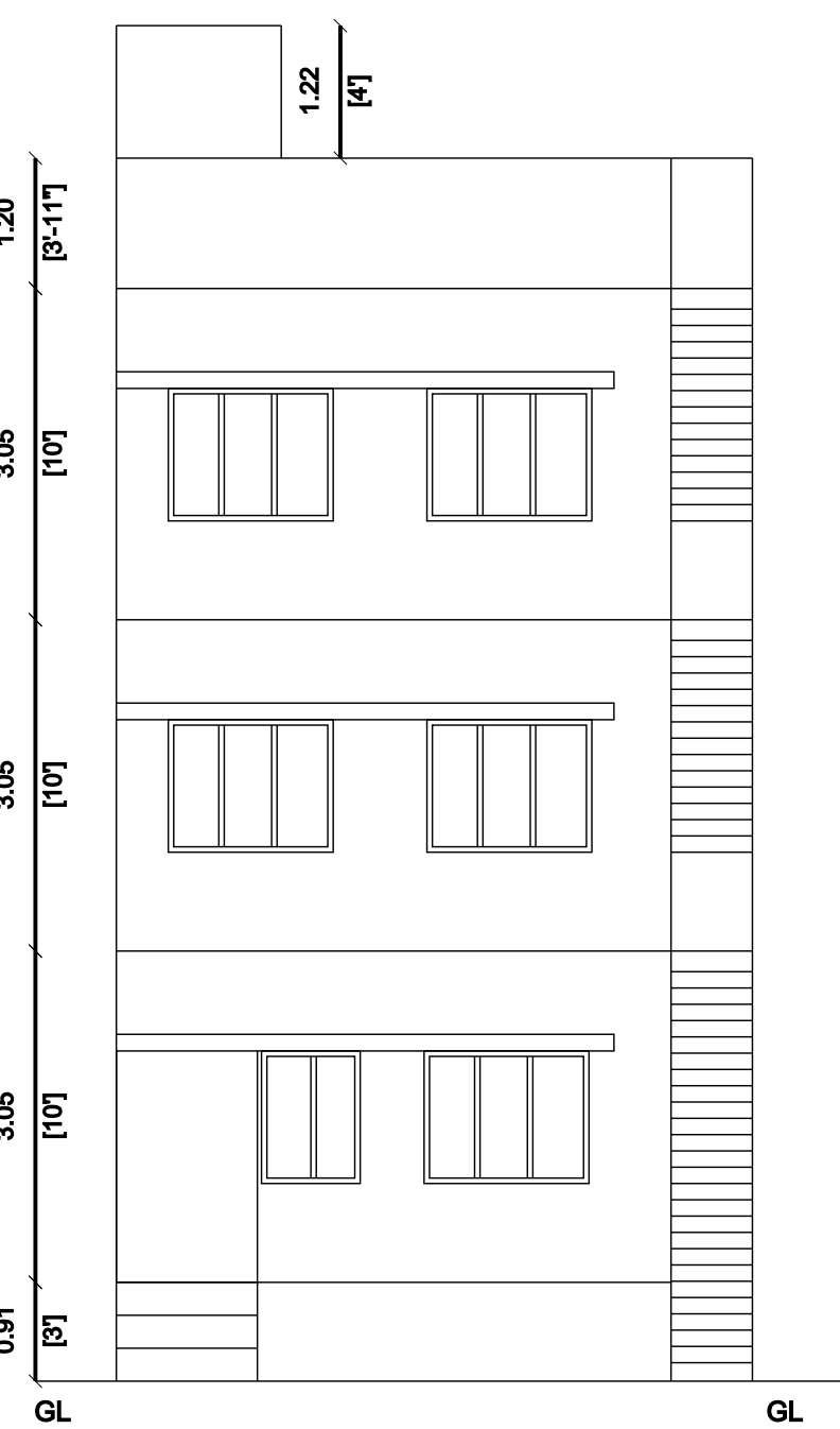
FRONT ELEVATION
