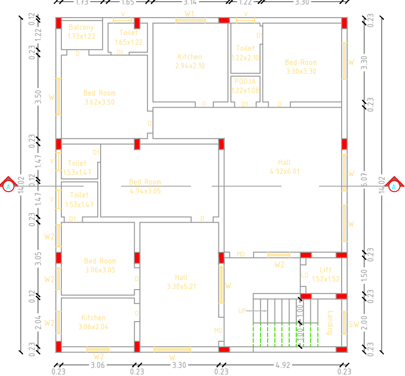
TYPICAL FLOOR PLAN FIRST & SECOND
