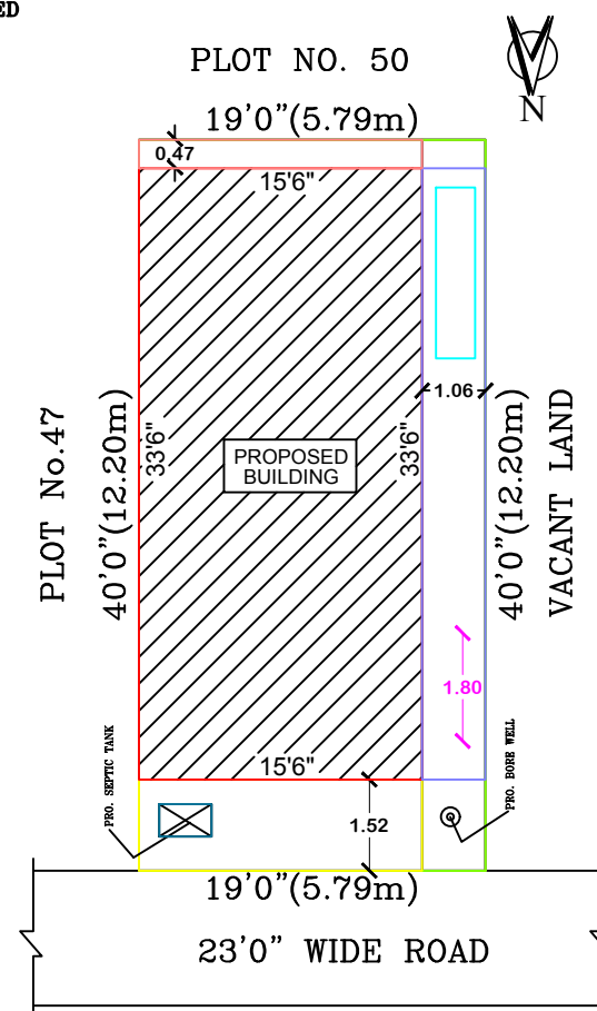
SITE PLAN
