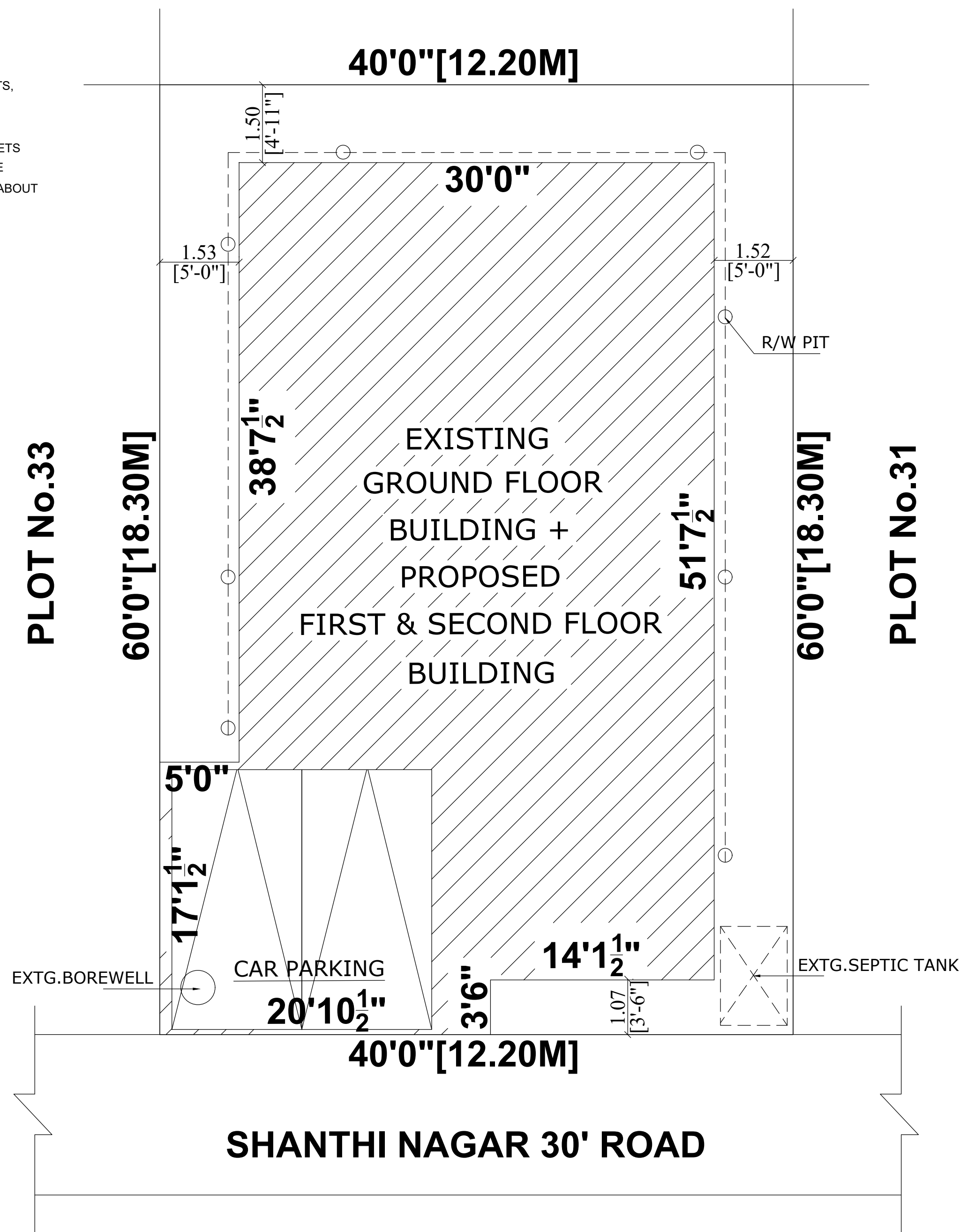
SITE PLAN
