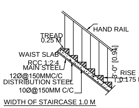
WIDTH OF STAIRCASE 1.0 M
