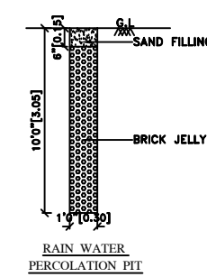
RAIN WATER COLLECTION SYSTEM
