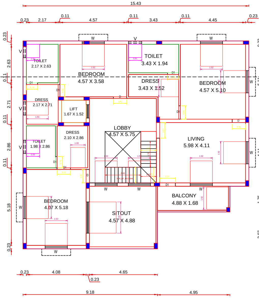
FIRST FLOOR PLAN (PROPOSED)
