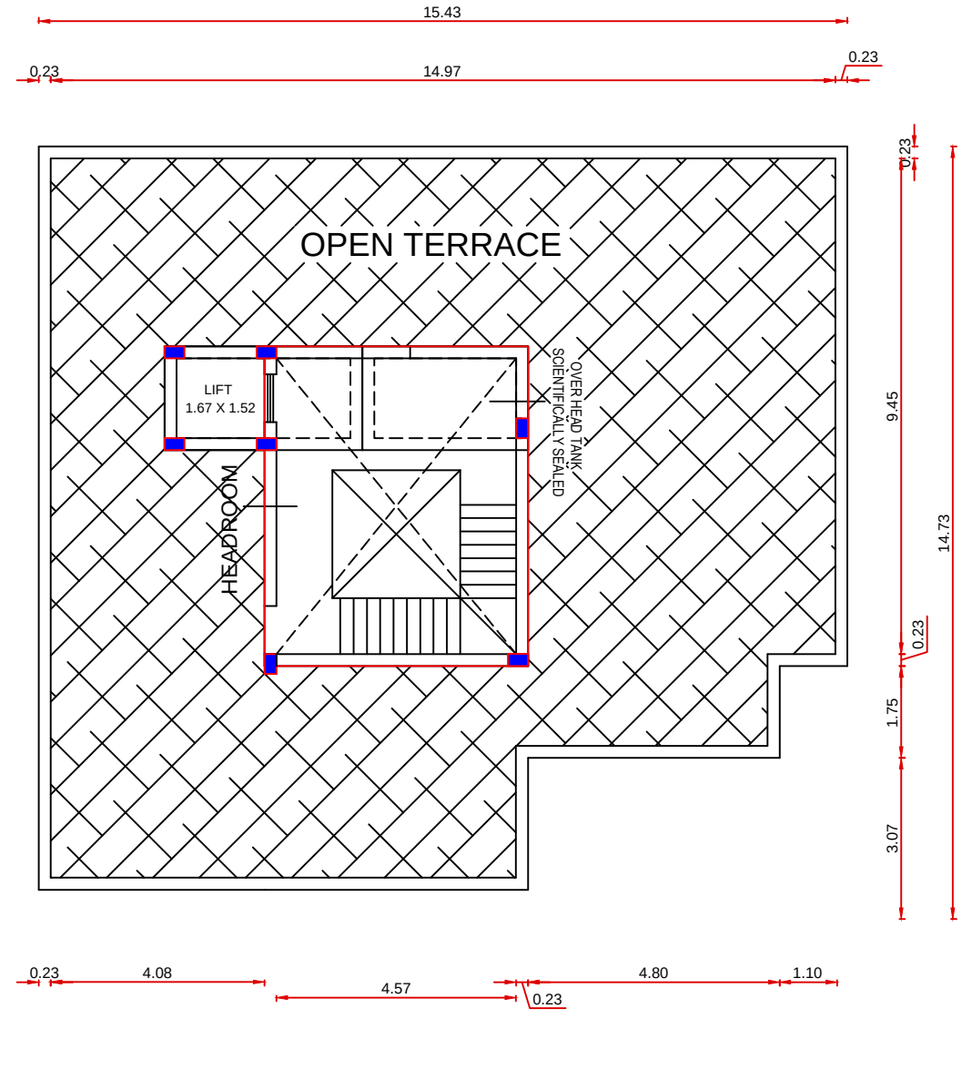
TERRACE FLOOR PLAN (PROPOSED)
