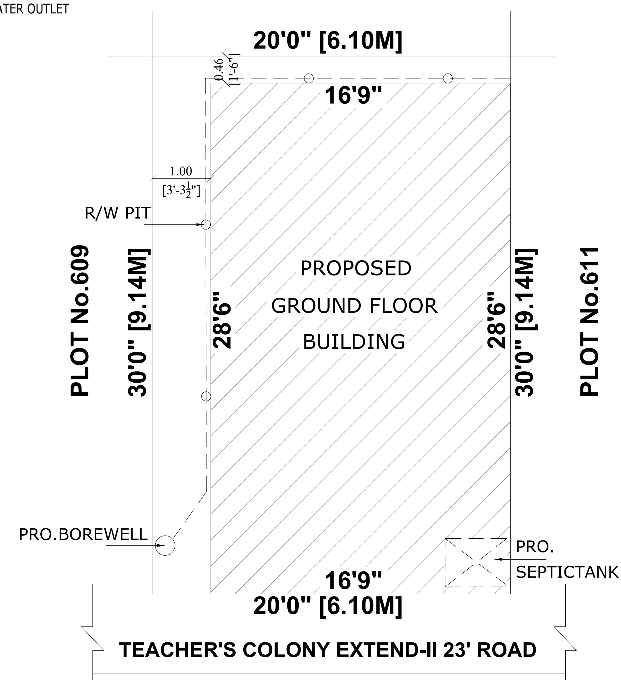
SITE PLAN
