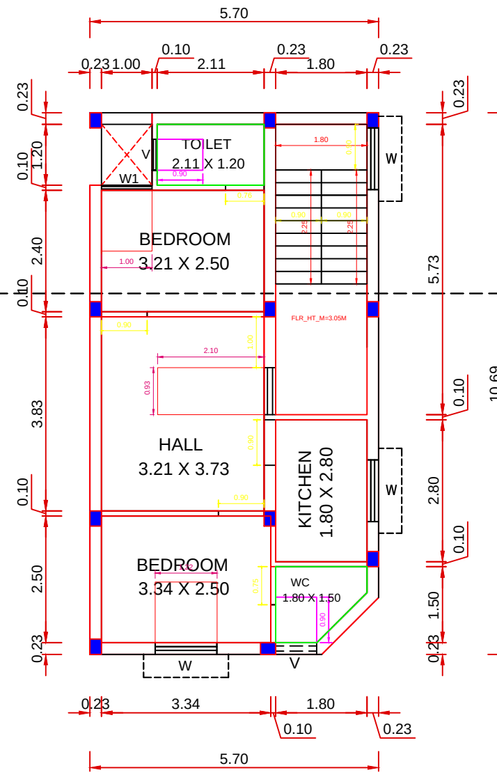
FIRST FLOOR PLAN (PROPOSED)
