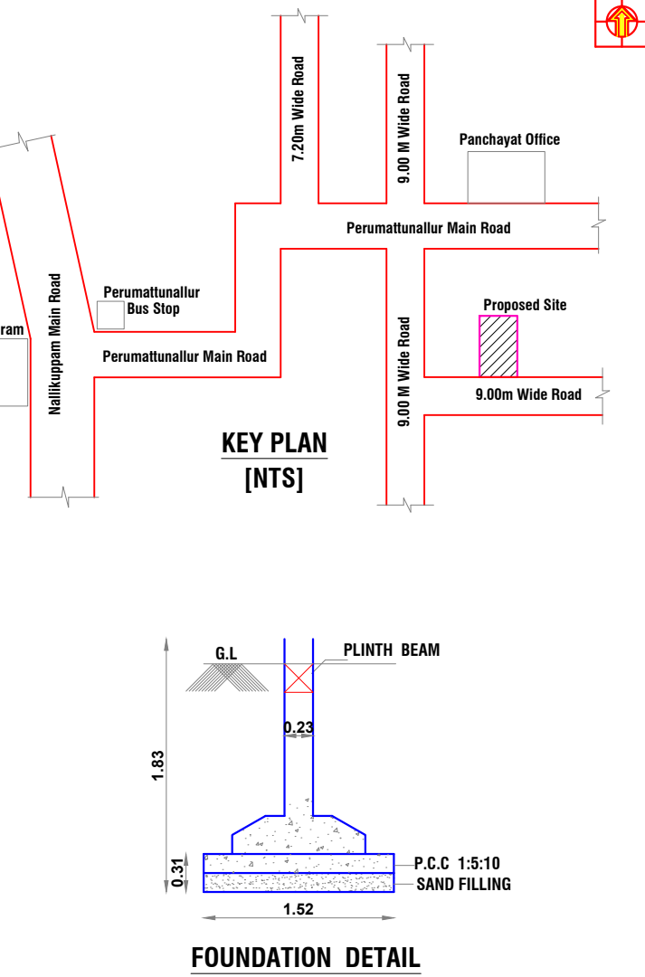
FOUNDATION DETAIL
