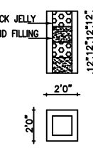
PERCOLATION PIT
