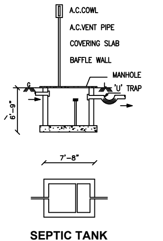
SEPTIC TANK
