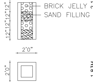
PERCOLATION PIT
