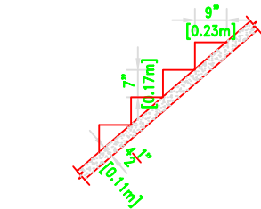
STAIRCASE DETAIL
