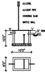
SEPTIC TANK DETAILS
