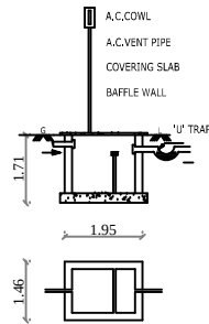
SEPTIC TANK
