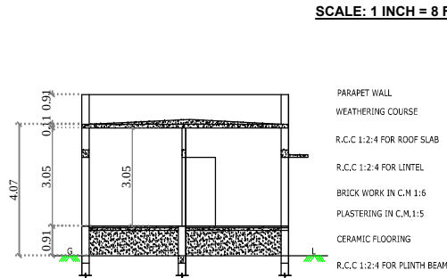
SECTION ON "SC"
