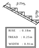
STAIRS DETAILS
