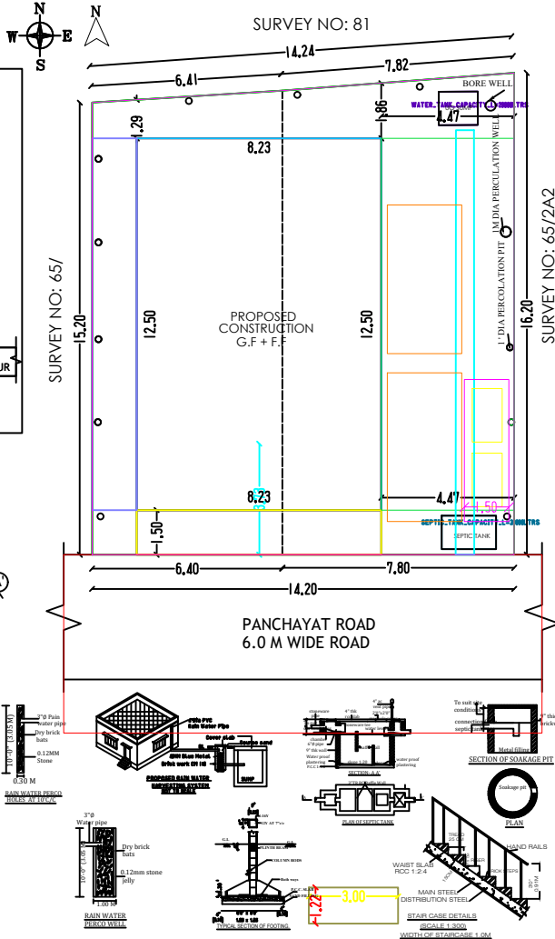
KEY PLAN SCALE 1:100
