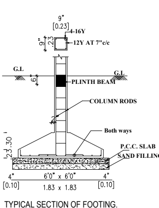
TYPICAL SECTION OF FOOTING.
