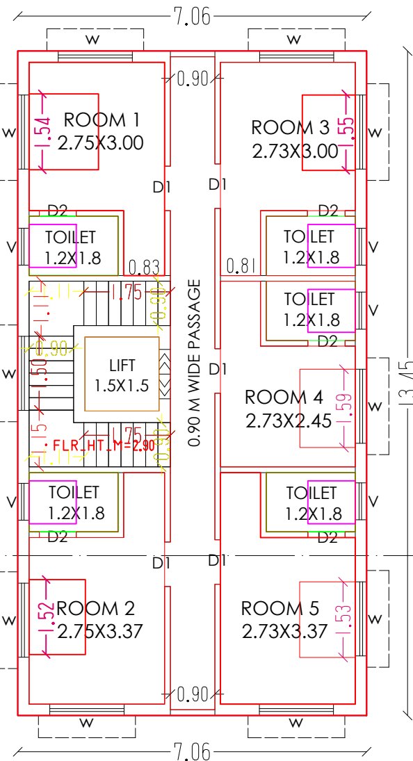
SECOND FLOOR PLAN SCALE 1:100
