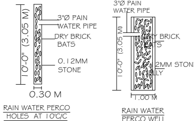
RAIN WATER PERCO TILES AT 10°C
