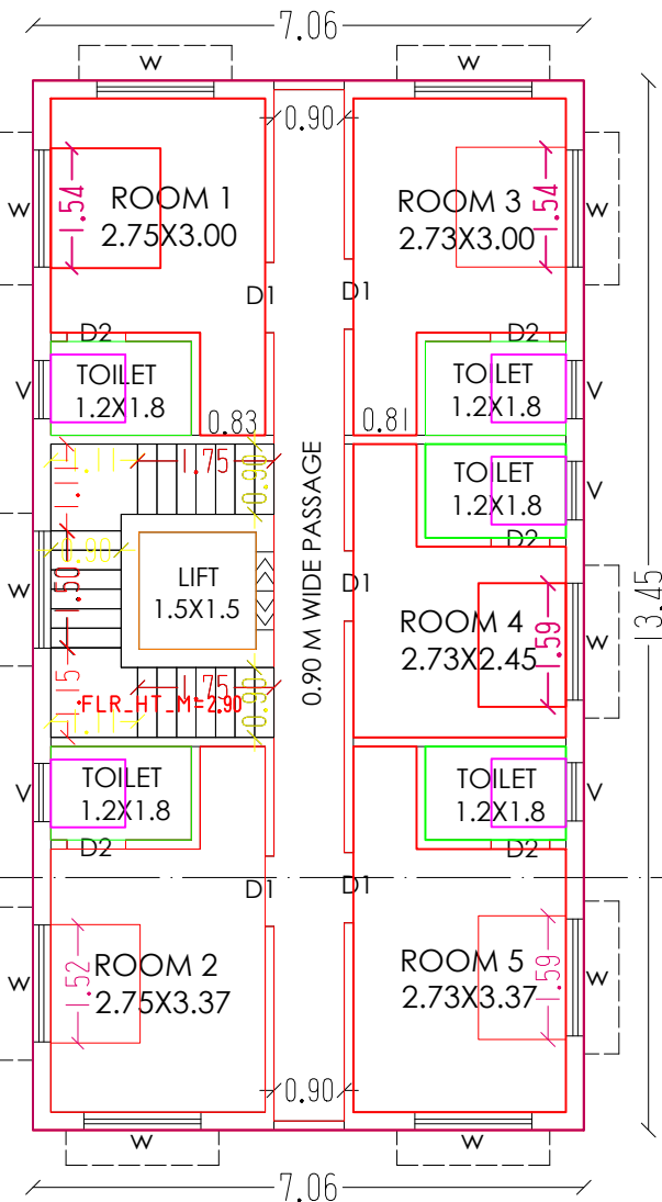
THIRD FLOOR PLAN SCALE 1:100
