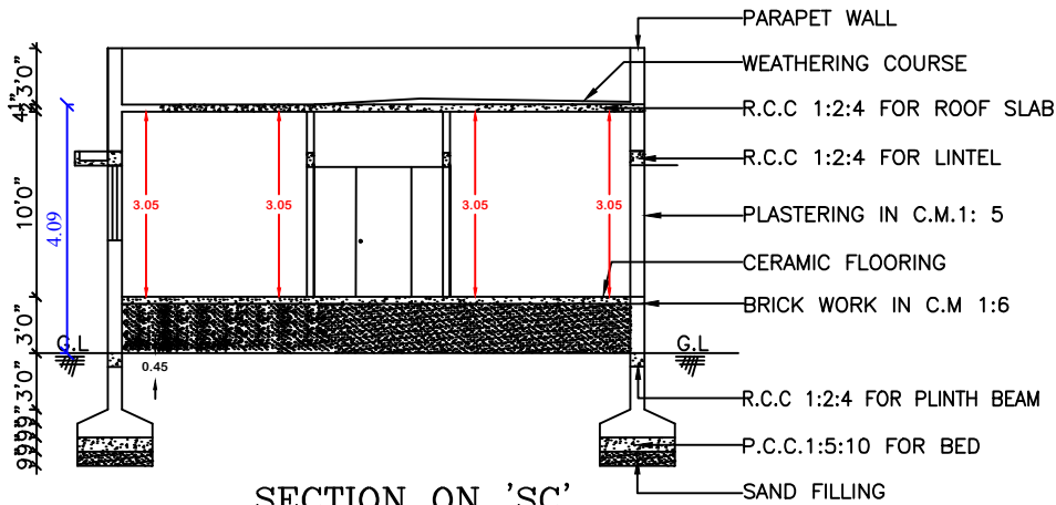
SECTION ON 'SC'
