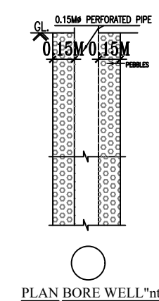
PLAN BORE WELL"nts"
