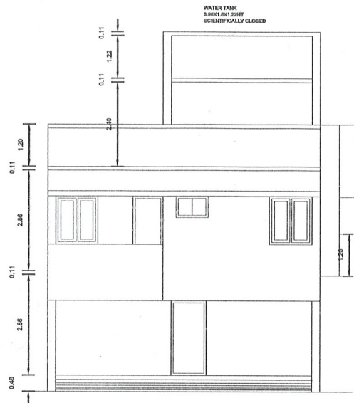
FRONT ELEVATION
