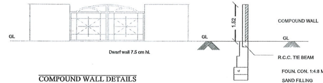
COMPOUND WALL DETAILS
