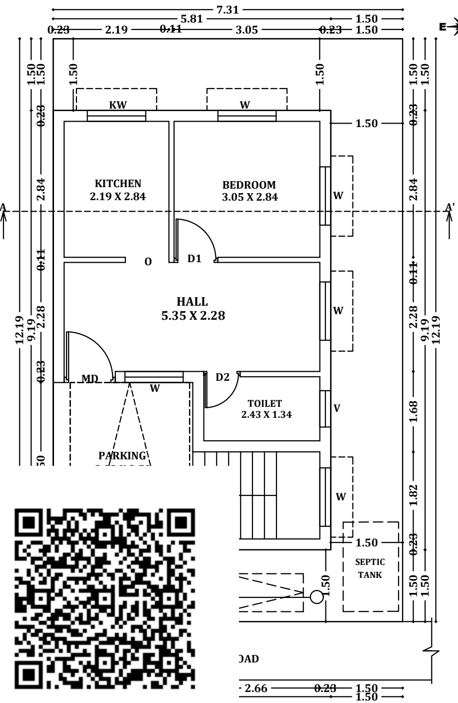
D FLOOR PLAN
