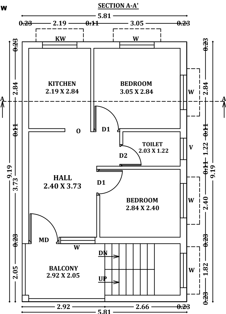
FIRST & SECOND FLOOR PLAN TYPICAL FLOOR PLAN
