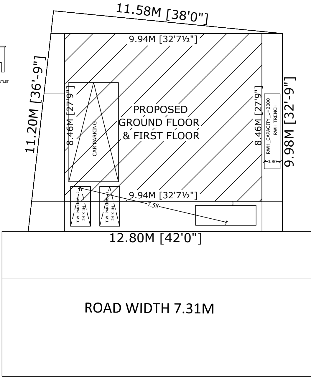
SITE PLAN
