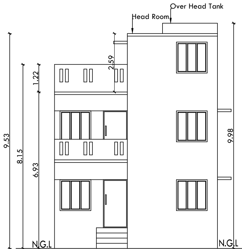
Front Elevation
