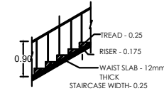
STAIR CASE DETAIL
