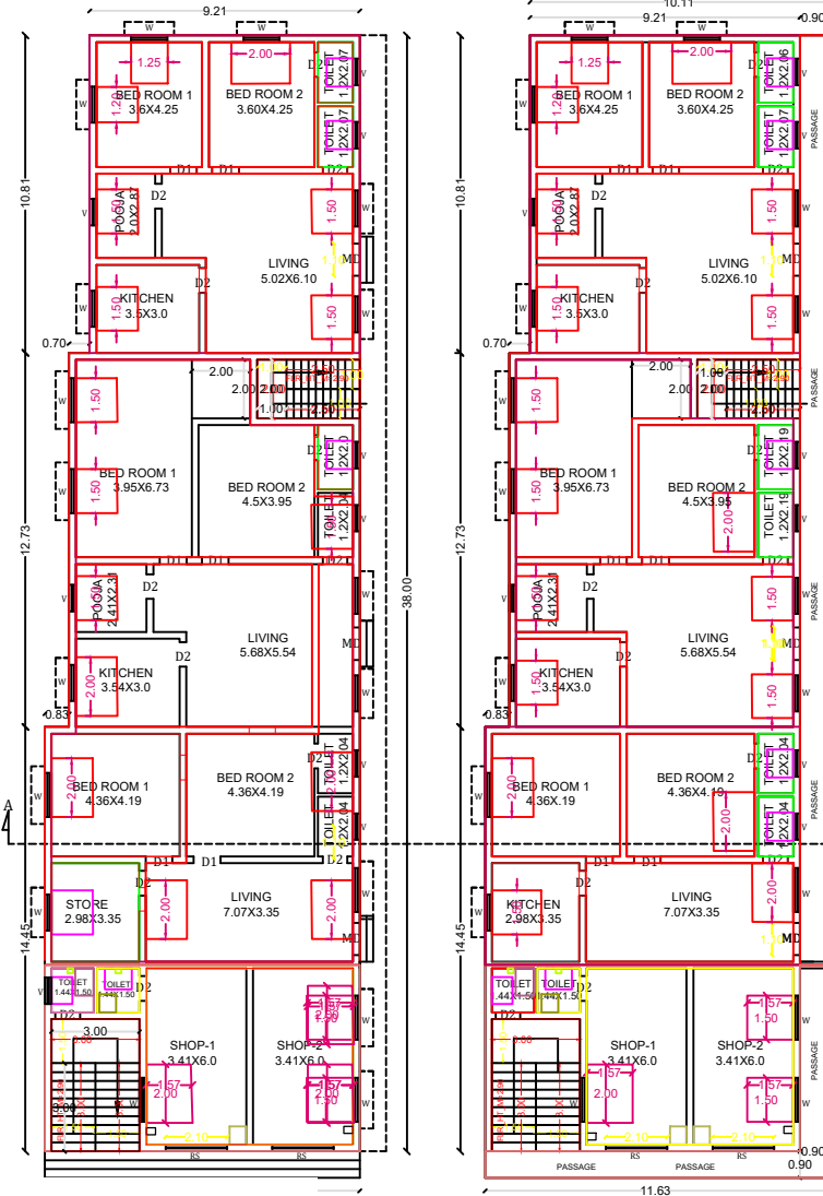
FIRST FLOOR SCALE 1:100
