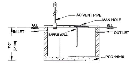
SECTION ON SEPTIC TANK
