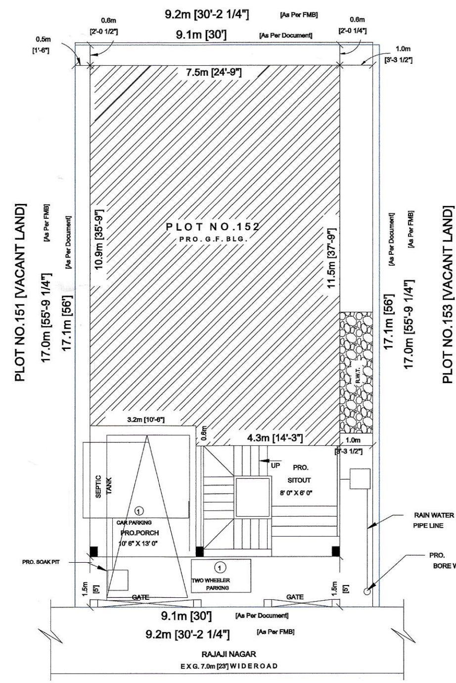
SITE PLAN
