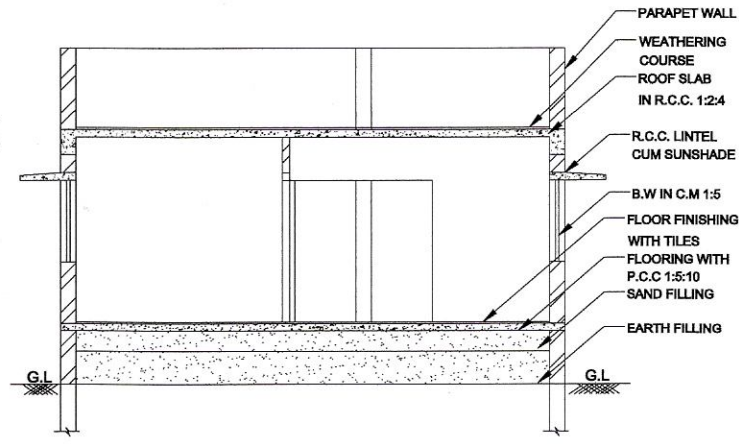
SECTION ON "JS"
