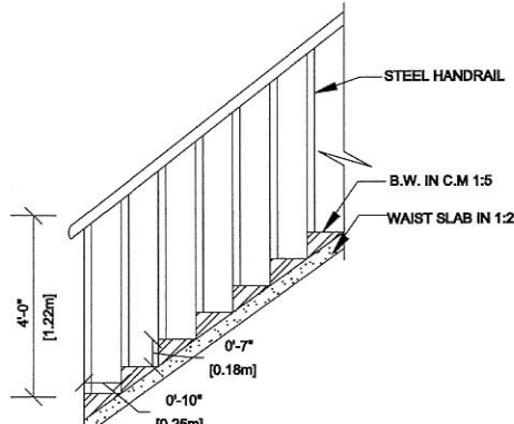
STAIRCASE DETAILS SCALE 1:50
