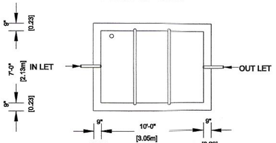
PLAN OF SEPTIC TANK [SCALE 1:50]
