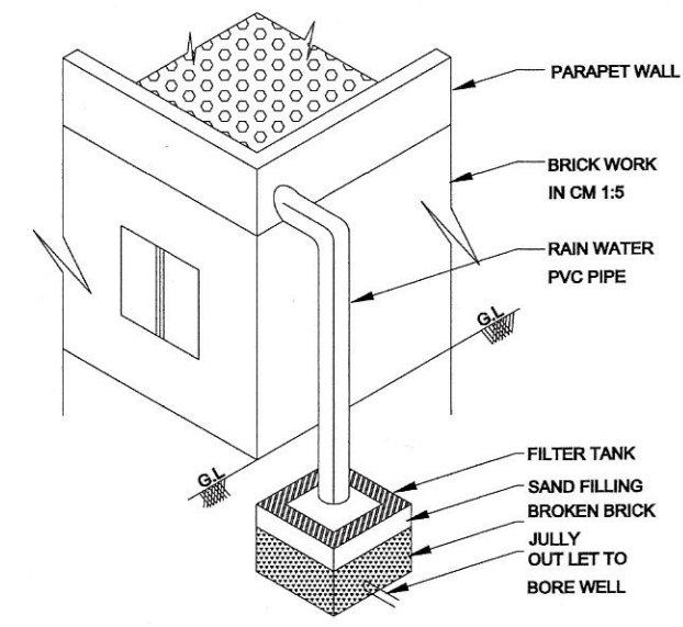
RAIN WATER HARVEST SYSTEM [NTS]
