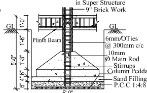
FOUNDATION DETAIL
