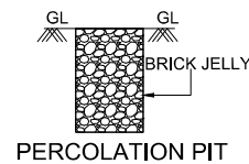
PERCOLATION PIT
