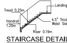
STAIRCASE DETAIL
