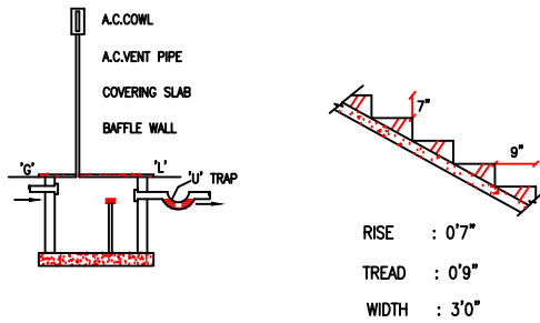
STAIRS DETAILS
