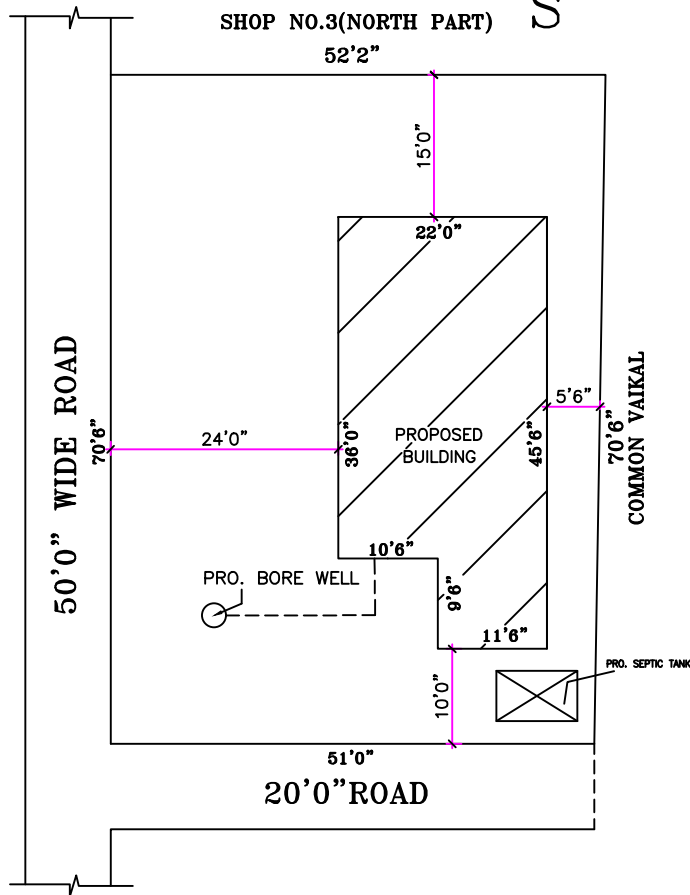
SITE PLAN
