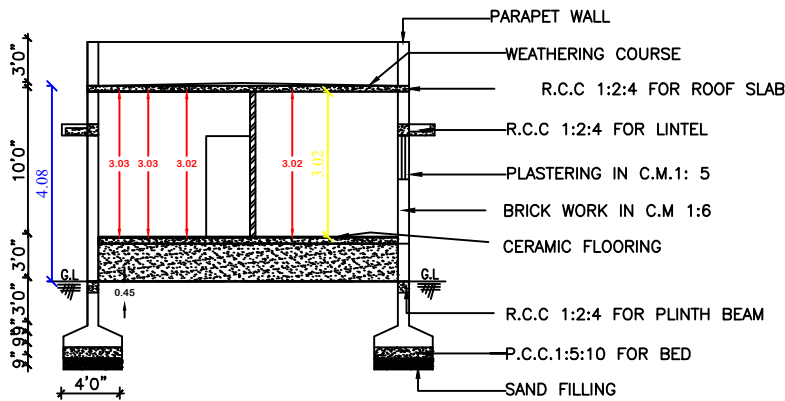
SECTION ON 'SC'
