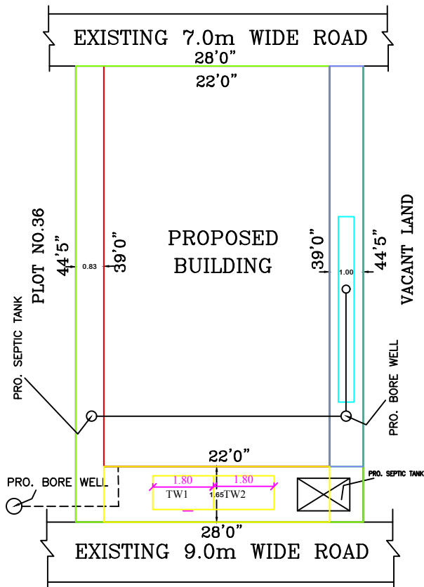
SITE PLAN
