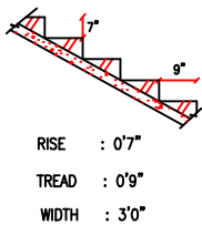
STAIRS DETAILS
