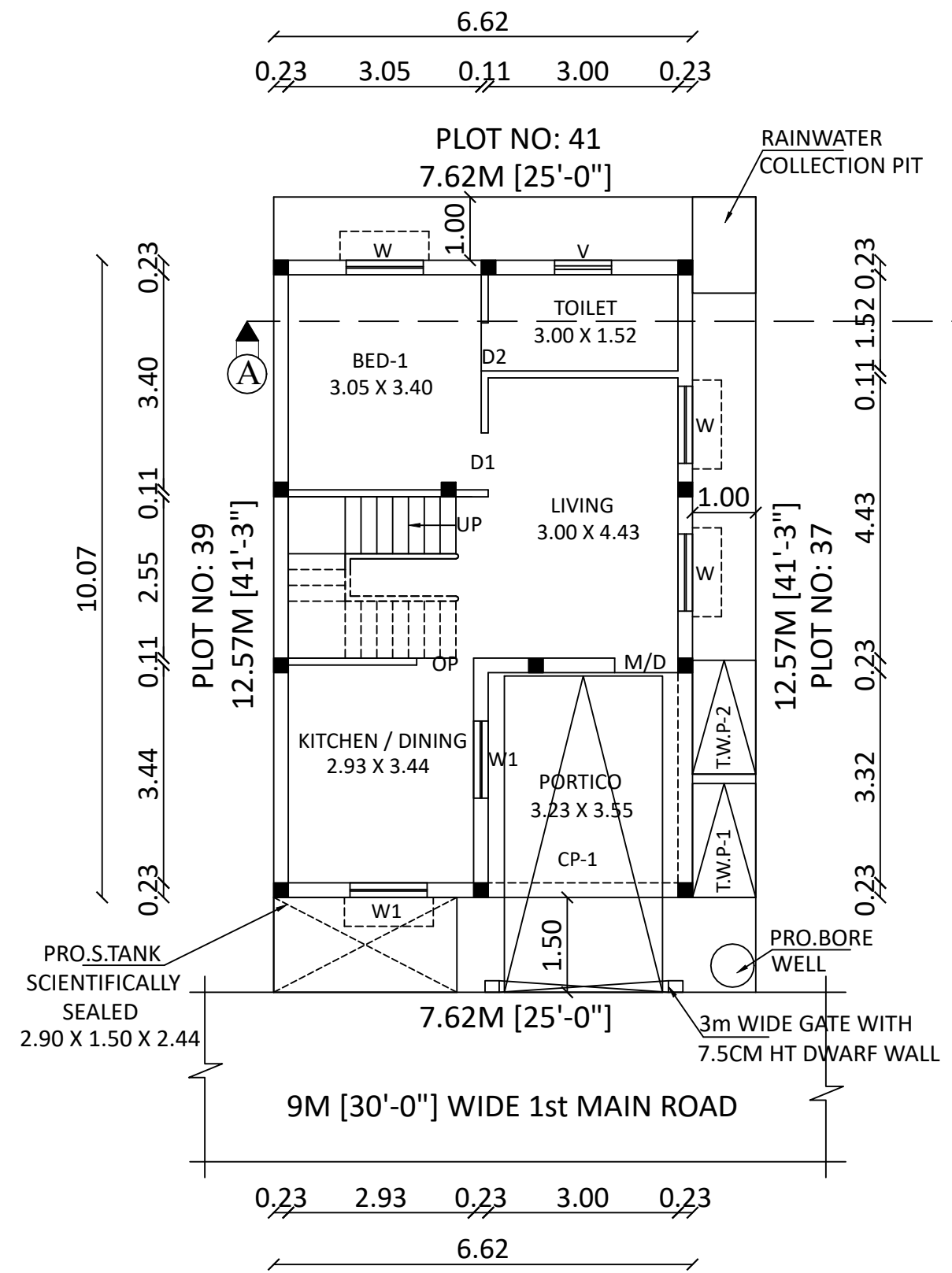
SITE CUM PRO.GROUND FLOOR PLAN
