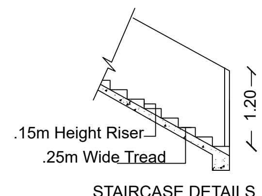
STAIRCASE DETAILS
