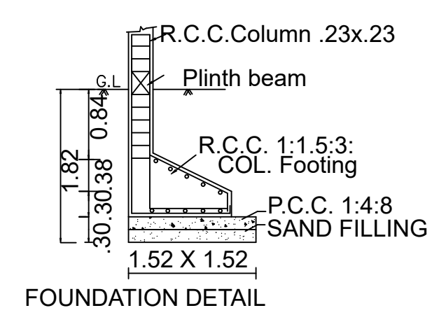
FOUNDATION DETAIL
