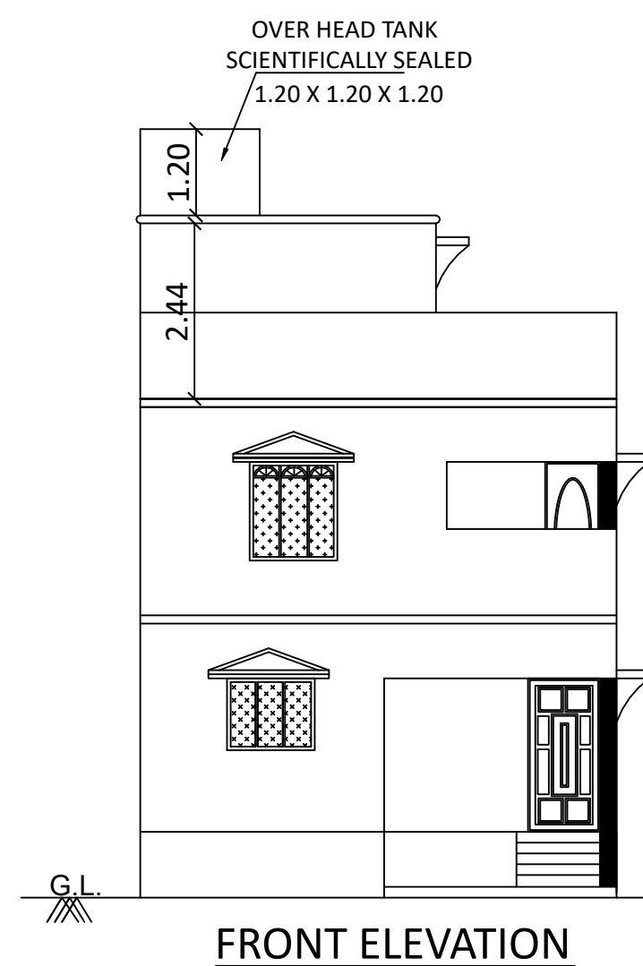
FRONT ELEVATION
