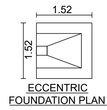
FOUNDATION DETAIL
