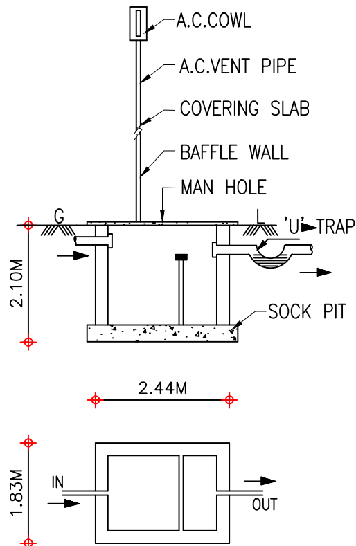
SEPTIC TANK
