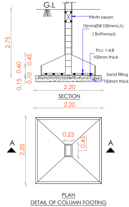
DETAIL OF COLUMN FOOTING
