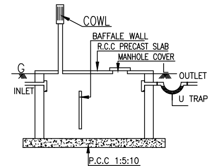
SECTION DETAILS OF SEPTIC TANK
