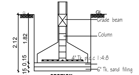
SECTION
