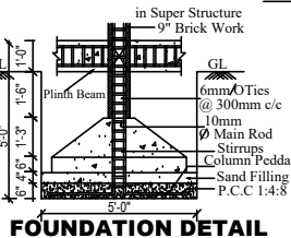
FOUNDATION DETAIL
