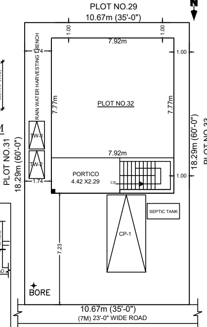
SITE PLAN (SCALE:1:100)
