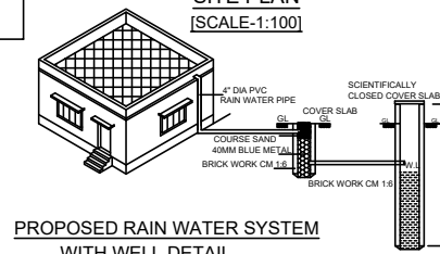
CROSS SECTION OF WELL 4'0" DIA
