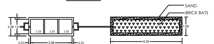
SEPTIC TANK AND TRENCH
