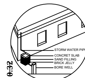
DETAIL RAINWATER HARVESTING
