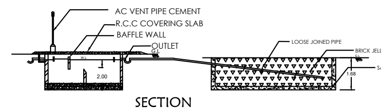
SECTION
