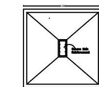
COLUMN FOUNDATION DETAIL PLAN OF FOOTING
