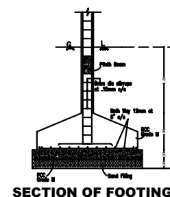
SECTION OF FOOTING
