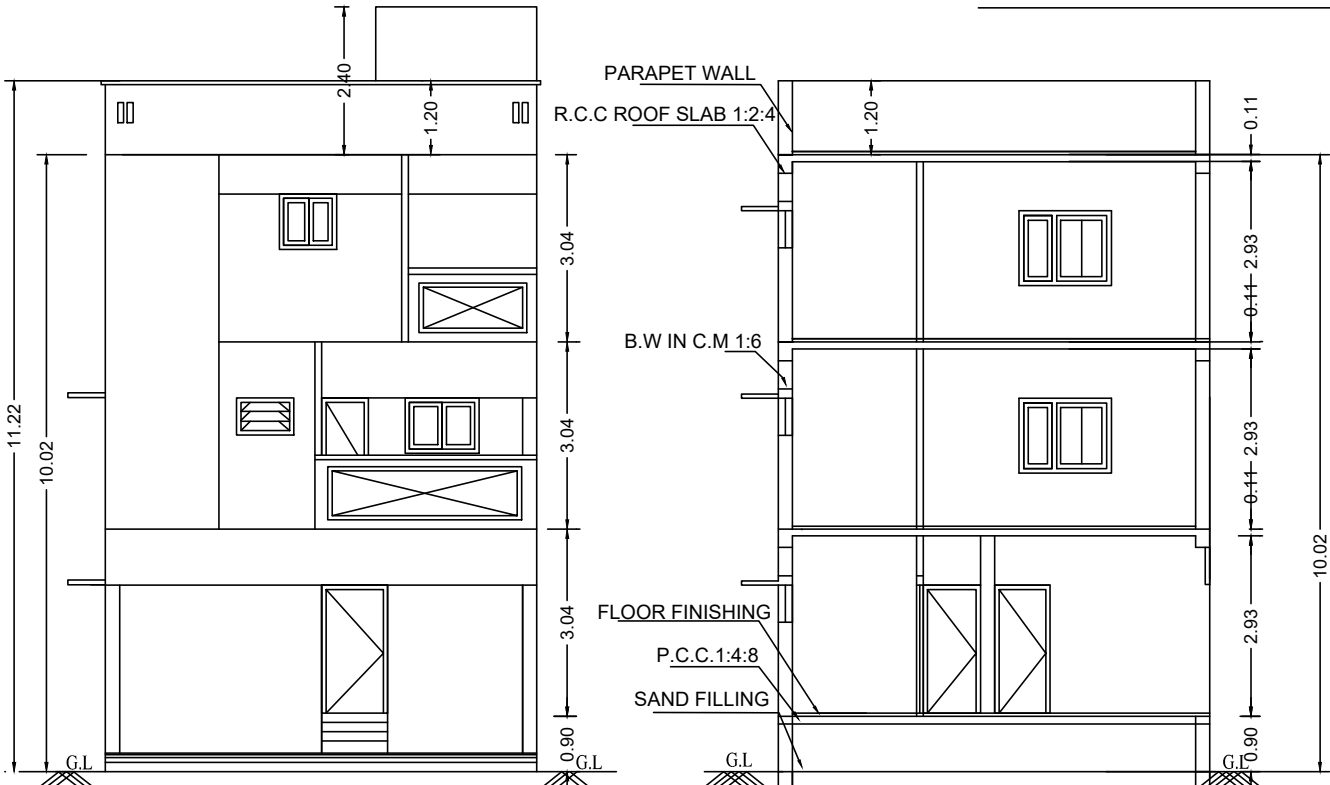
FRONT ELEVATION
