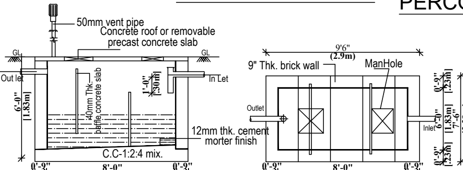
SECTION
