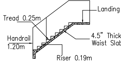
STAIRCASE DETAIL
