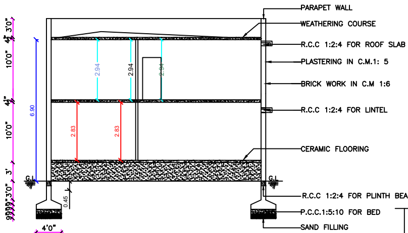
SECTION ON 'SC'
