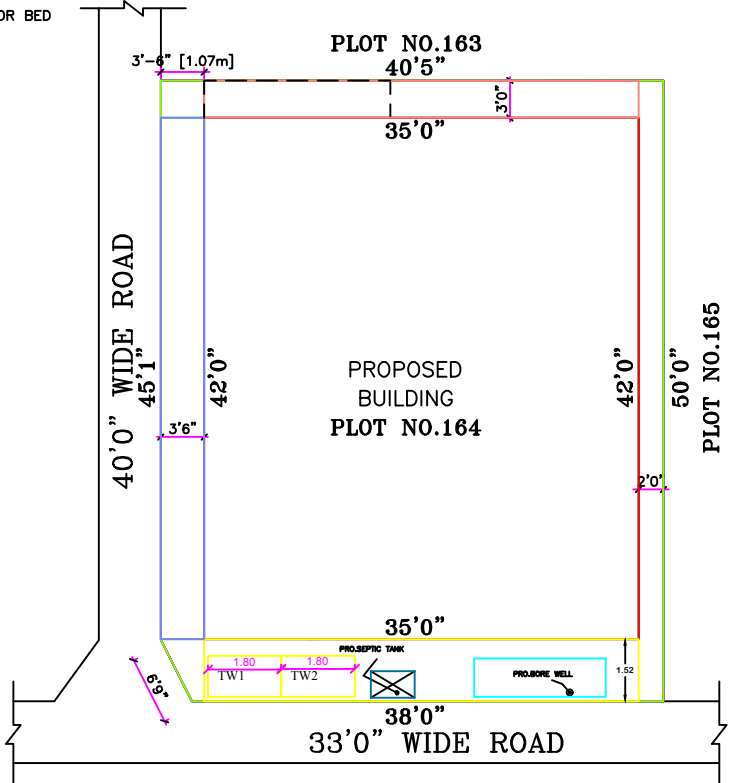
SITE PLAN
