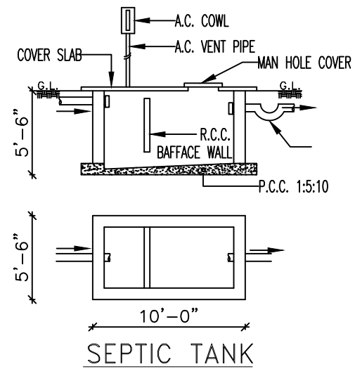
SEPTIC TANK
