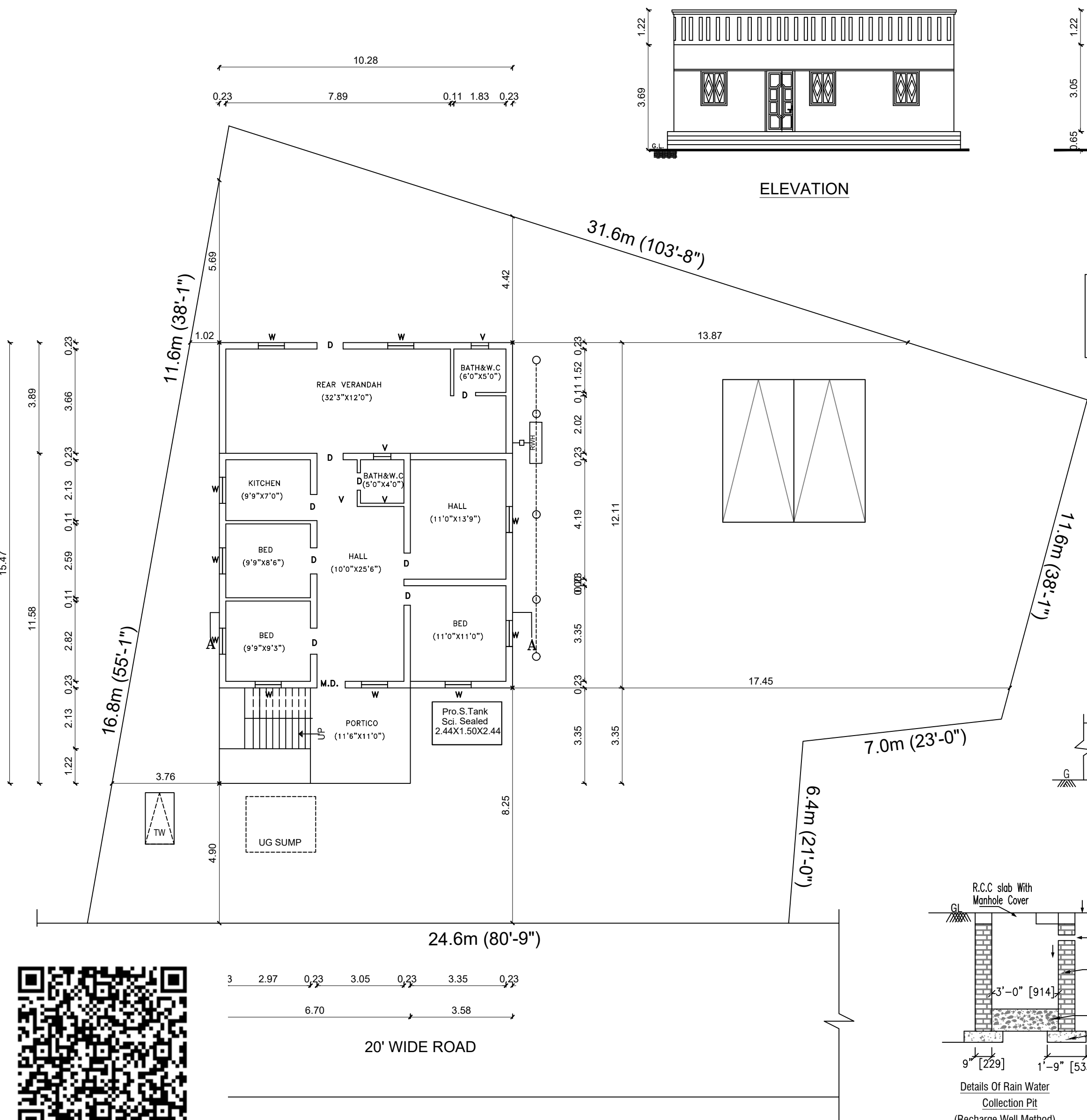
I / EXISTING & PROPOSED GROUND FLOOR PLAN (PROPOSED)
