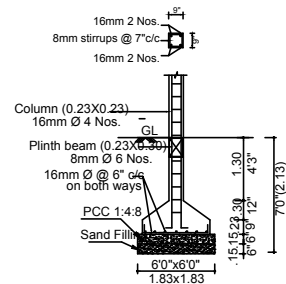
FOUNDATION DETAIL
