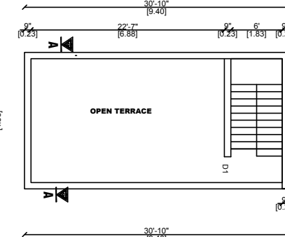
PROPOSED TERRACE FLOOR PLAN
