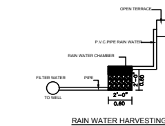
RAIN WATER HARVESTING
