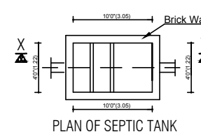
PLAN OF SEPTIC TANK
