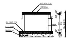
SECTION OF SUMP "X Y"
