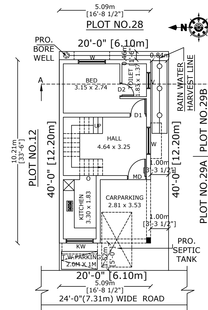
SITE CUM PRO. GROUND FLOOR PLAN
