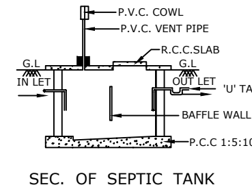
SEC. OF SEPTIC TANK
