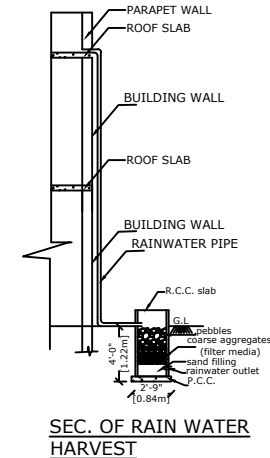
SEC. OF RAIN WATER HARVEST
