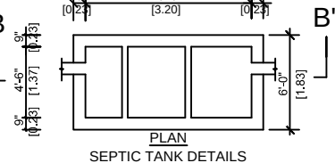
PLAN SEPTIC TANK DETAILS
