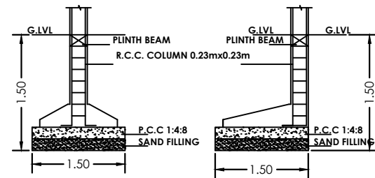
FOUNDATION DETAIL SCALE: 1.50
