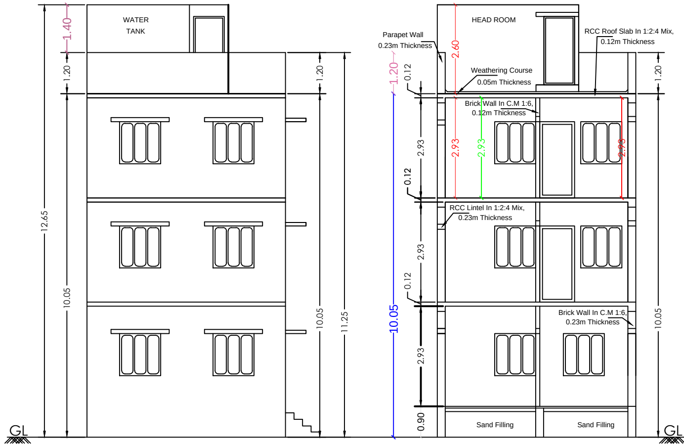
FRONT ELEVATION.
