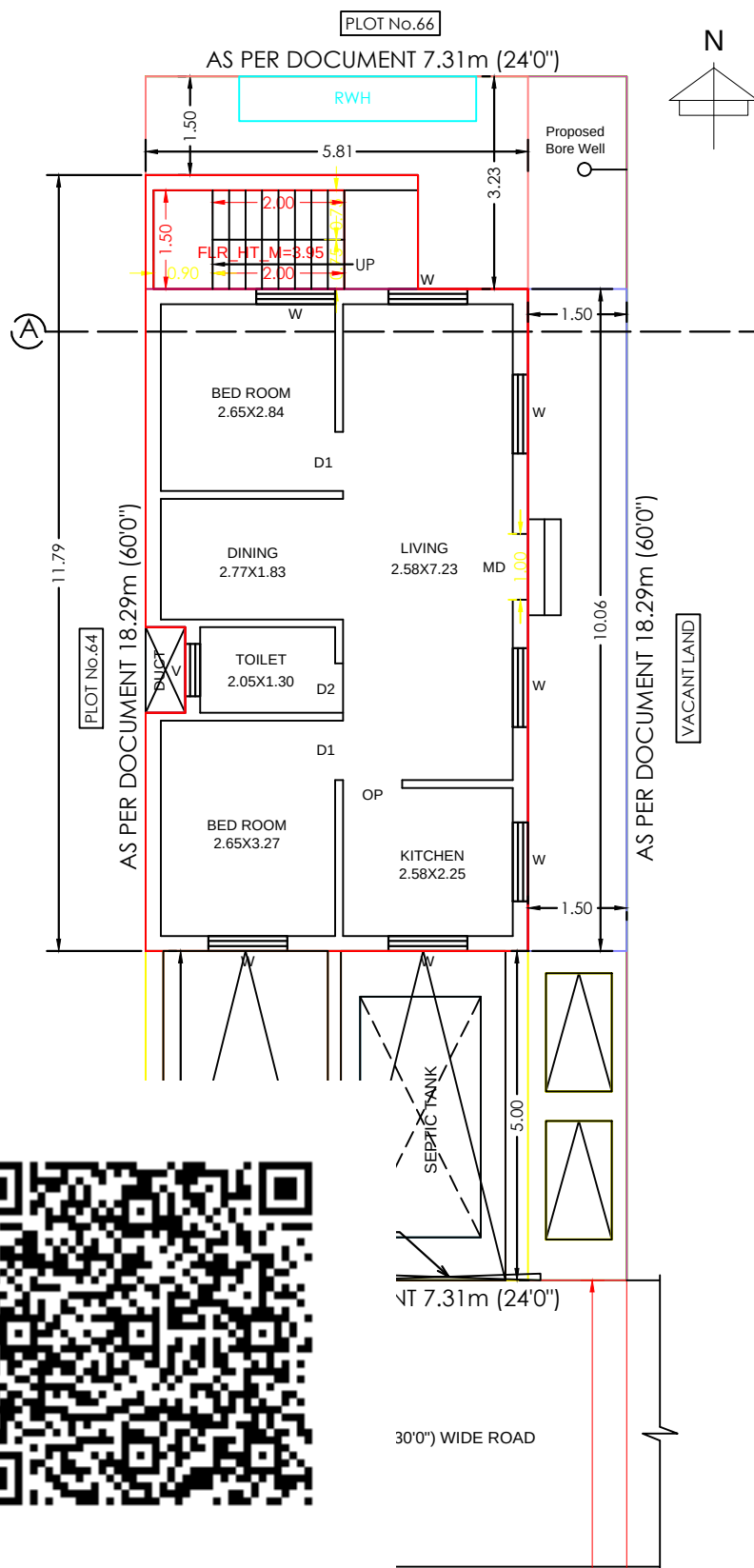
SITE / EXISTING GROUND FLOOR PLAN.
