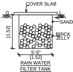
RAIN WATER FILTER TANK
