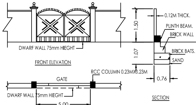
COMPOUND WALL & GATE DETAILS
