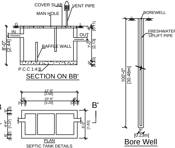
PLAN SEPTIC TANK DETAILS
