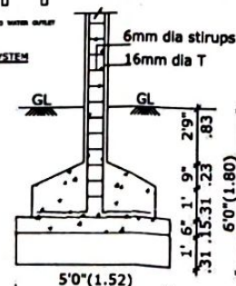
COLUMN FOUNDATION DETAIL SECTION OF BOREWELL
