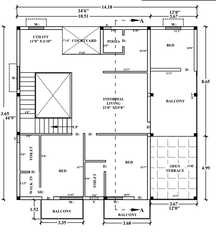
PLAN -EXG& PROPOSED( FIRST FLOOR)
