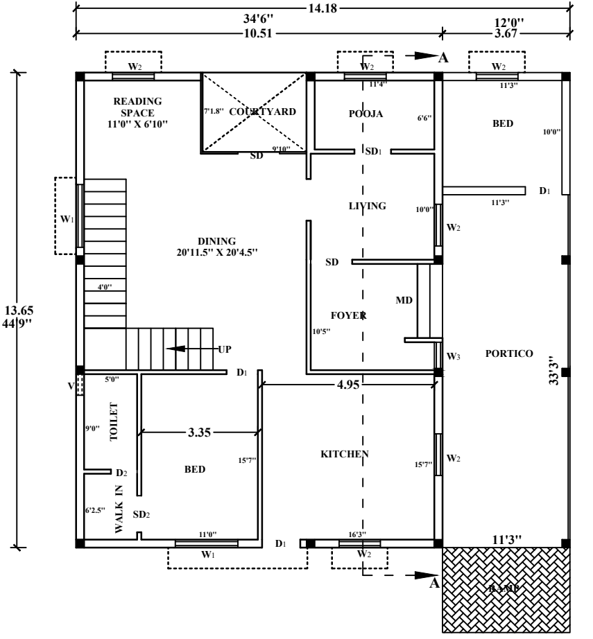
PLAN -EXG& PROPOSED ( GROUND FLOOR)
