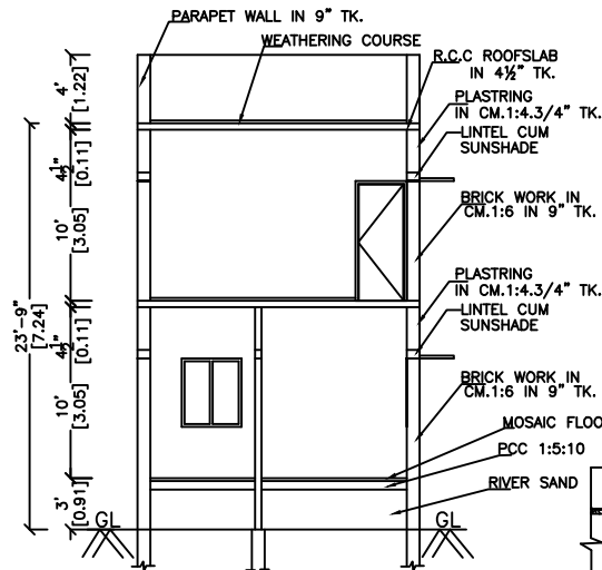
SECTION-"AB"
