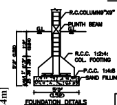
FOUNDATION DETAILS
