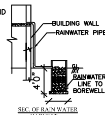
SEC. OF RAIN WATER HARVEST
