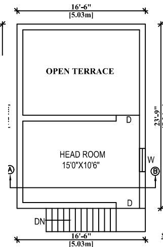
T(P) TERRACE(P) FLOOR PLAN
