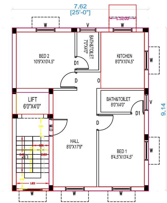
TYPICAL I, II & III- rd FLOOR PLAN
