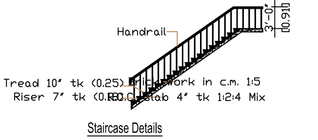
Staircase Details
