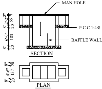
SEPTIC-TANK DETAIL
