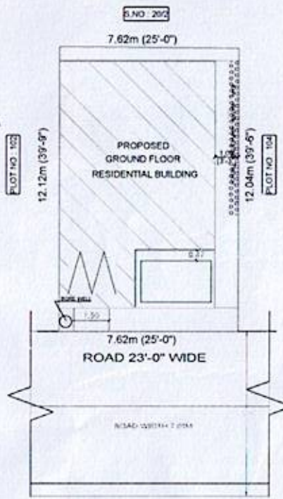
SITE PLAN (1:100)
