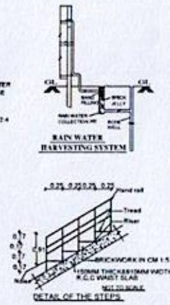
DETAIL OF THE STEPS
