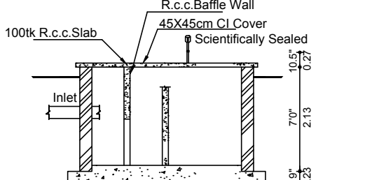
SECTION OF SEPTIC TANK "X Y"
