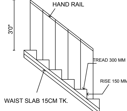
STAIR CASE DETAILS
