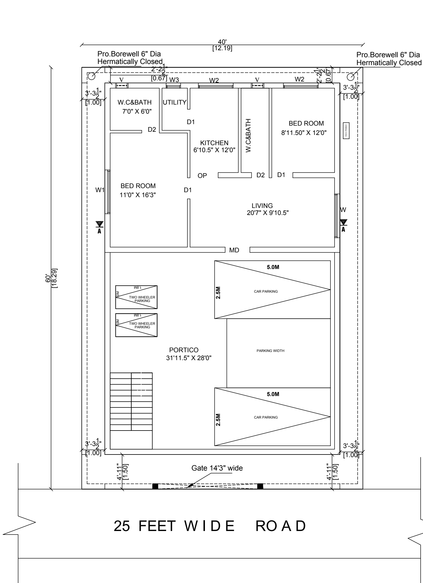
PROPOSED SITE CUM GROUND FLOOR PLAN
