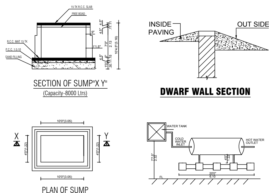
PLAN OF SUMP
