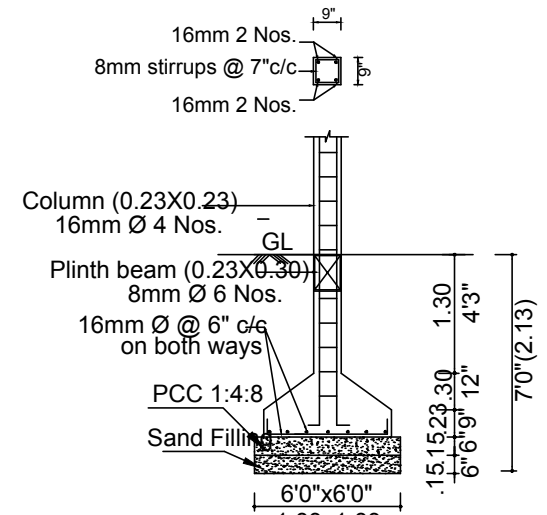
FOUNDATION DETAIL
