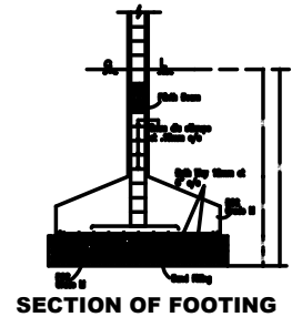
SECTION OF FOOTING
