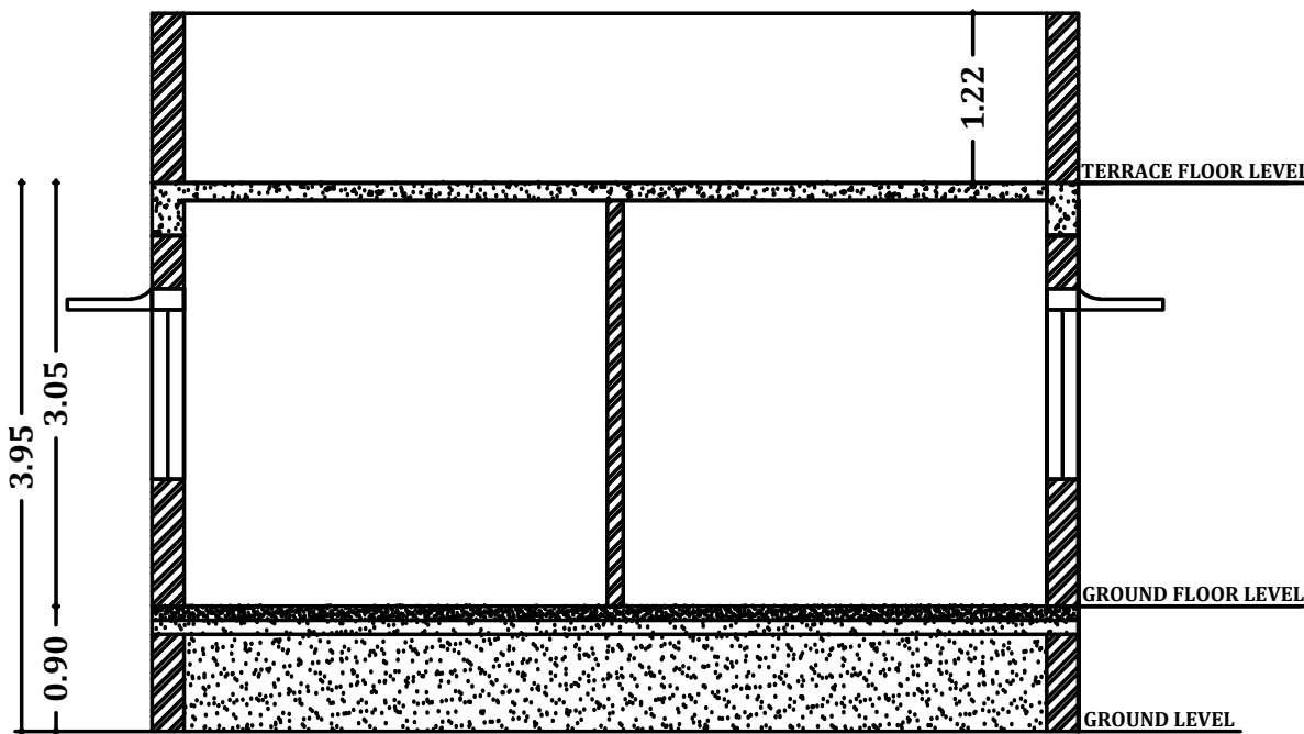
SECTION - AA'
