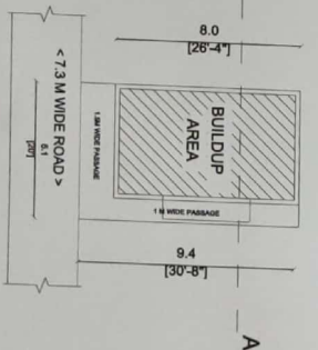
SITE CUM PROPOSED BUILDUP AREA
